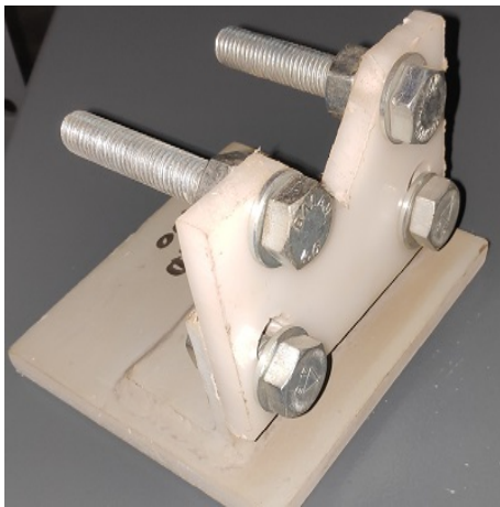
(a) PP Valve Support
